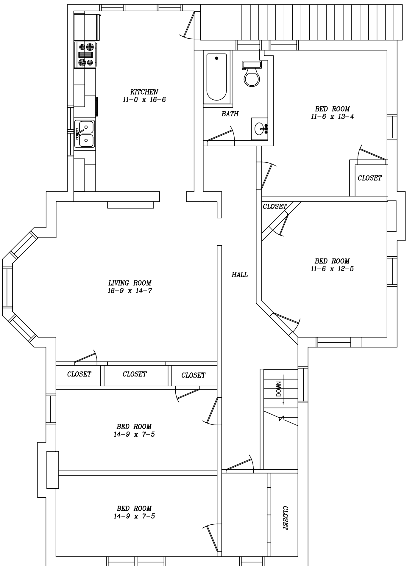
966 Vine Ave: Second Floor Not to Scale (Gr Liv Area 1295 sq ft)
