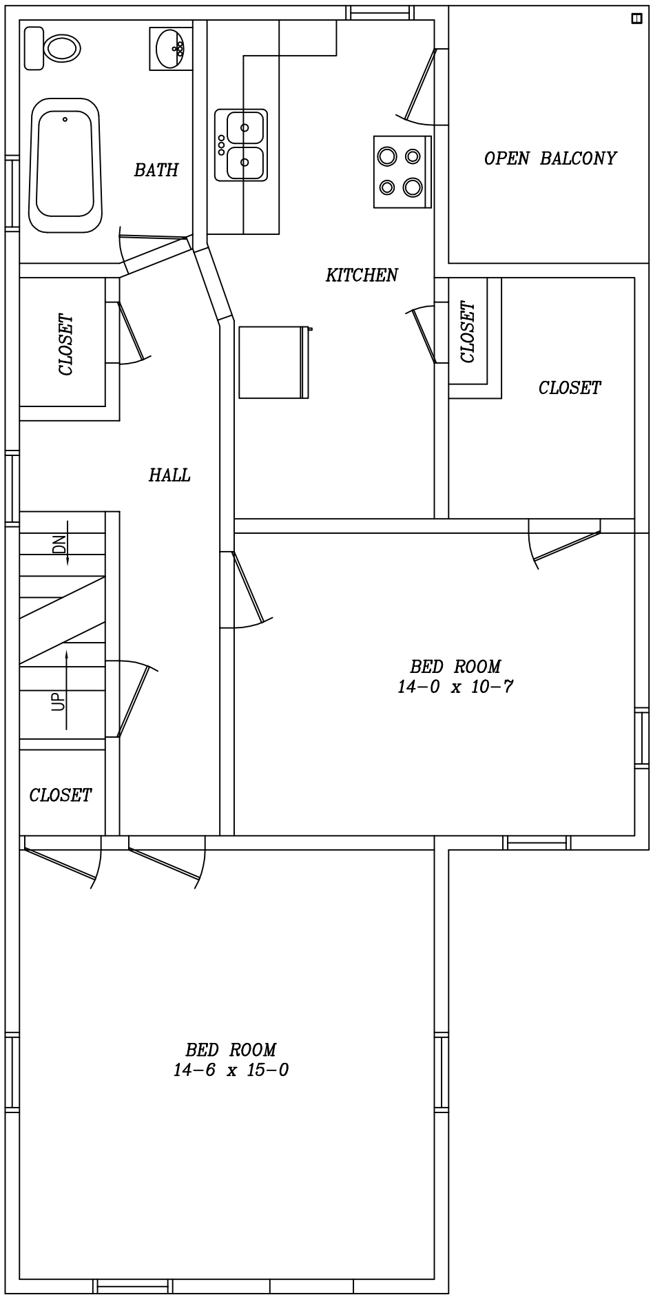
965 Vine Ave: Second Floor Not to Scale (Gr Liv Area 775 sq ft)
