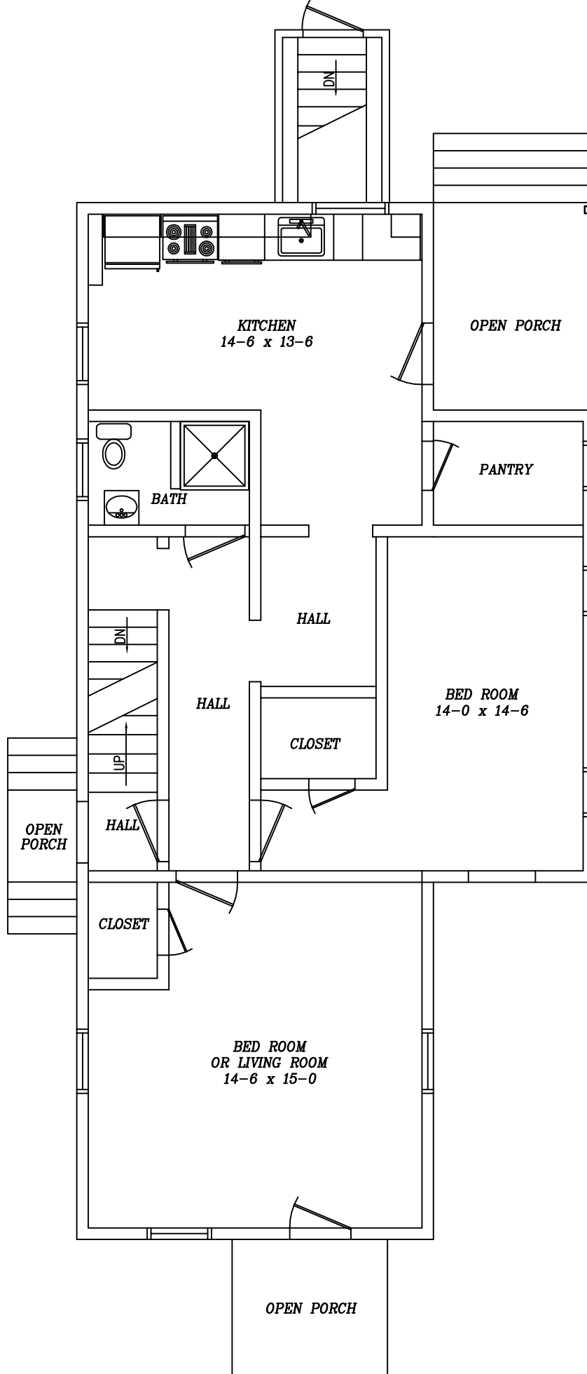
965 Vine Ave: First Floor Not to Scale (Gr Liv Area 775 sq ft)
