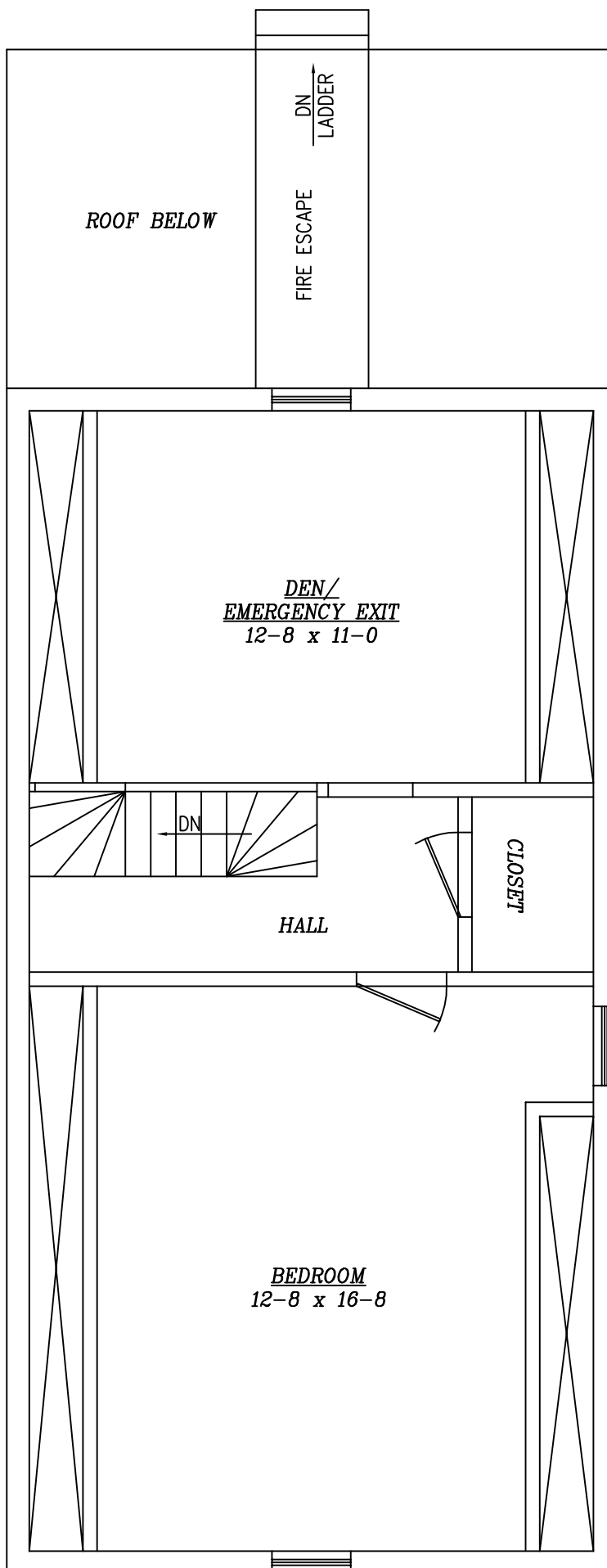
963 Vine Ave: Third Floor: Not to Scale (Gr Liv Area 440 sq ft)
