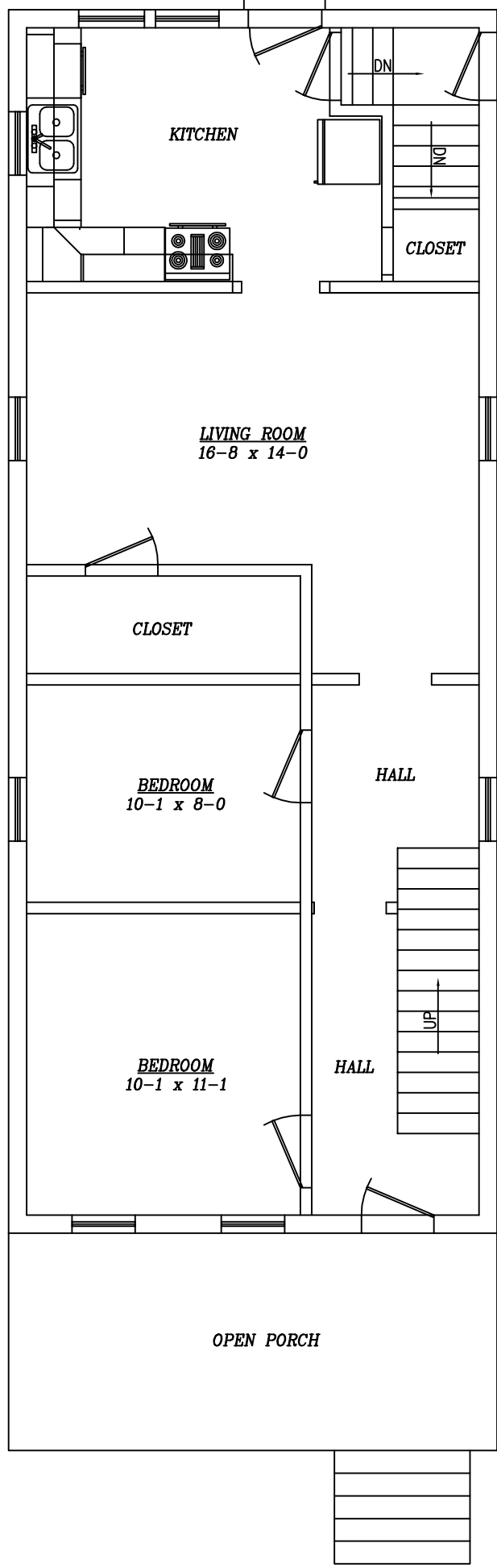
963 Vine Ave: First Floor Not to Scale (Gr Liv Area 730 sq ft)
