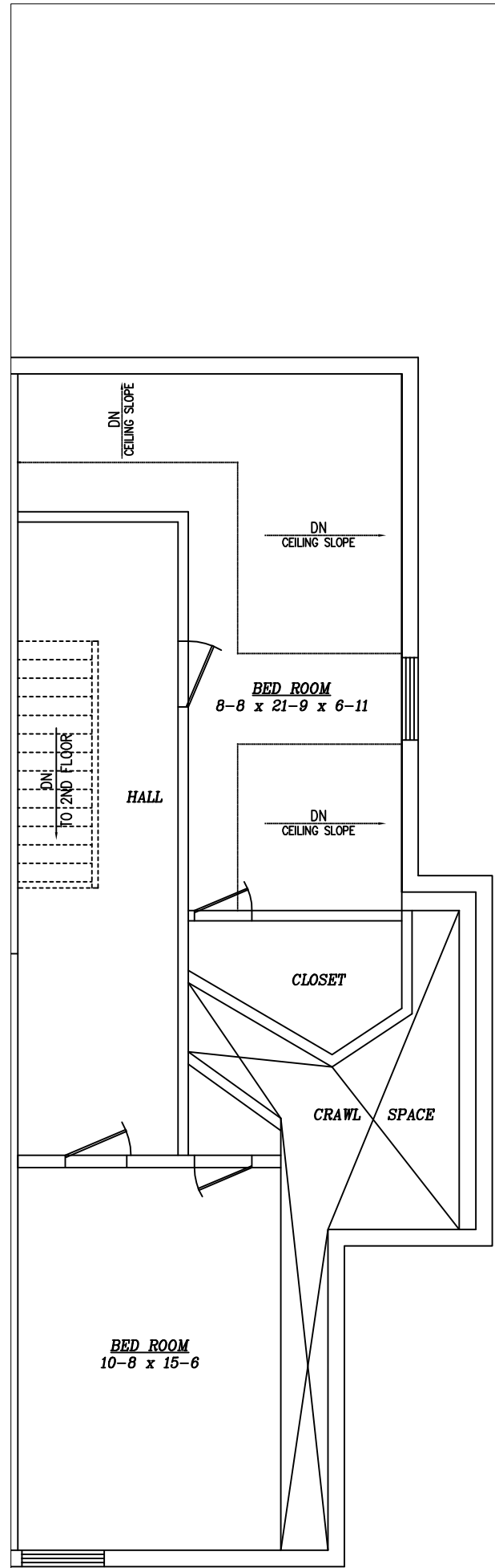
757 W Third St Apt. 2 (Third Floor) Not to Scale
