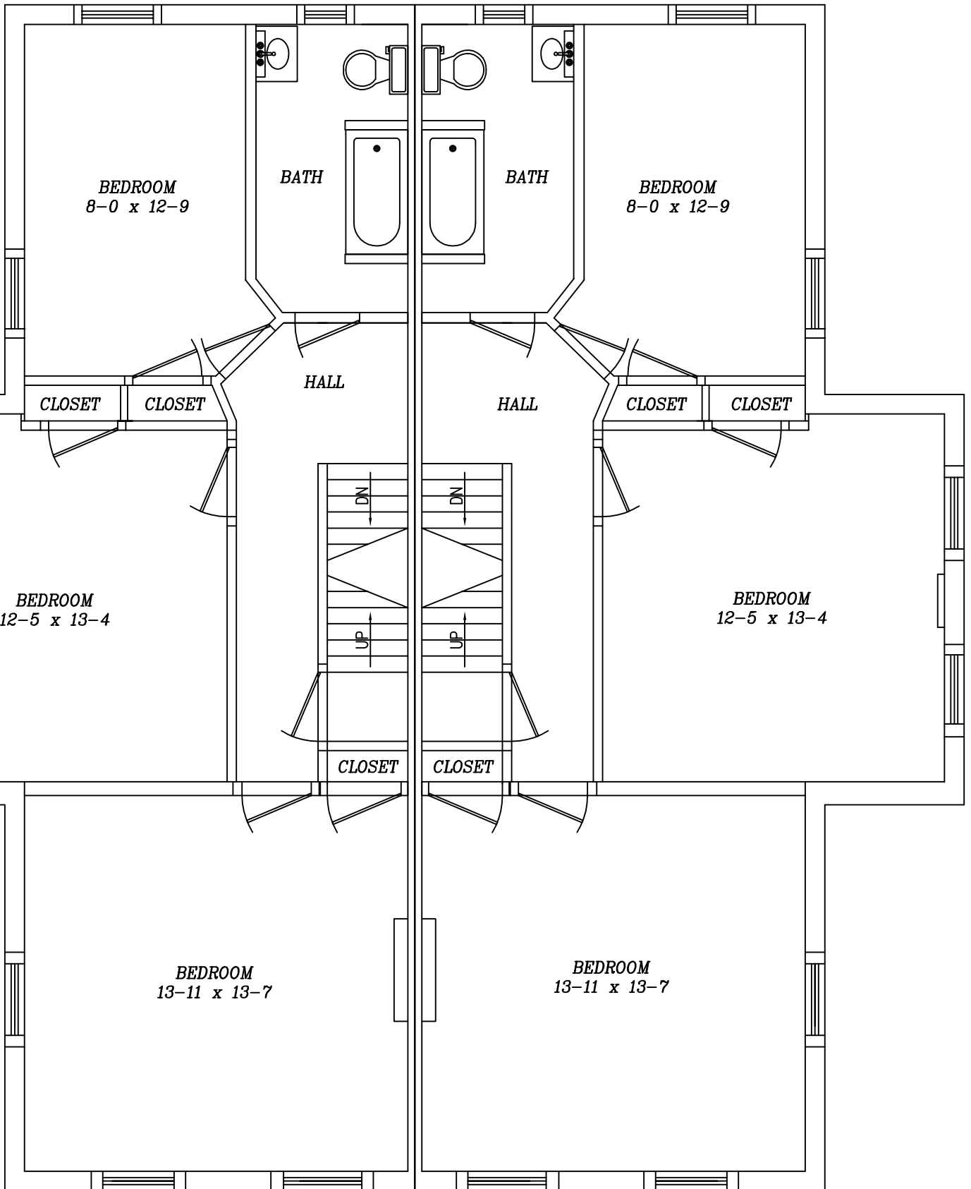
1020-1022 Vine Ave: Second Floor Not to Scale (Gross Living Area 1420 sq ft)
