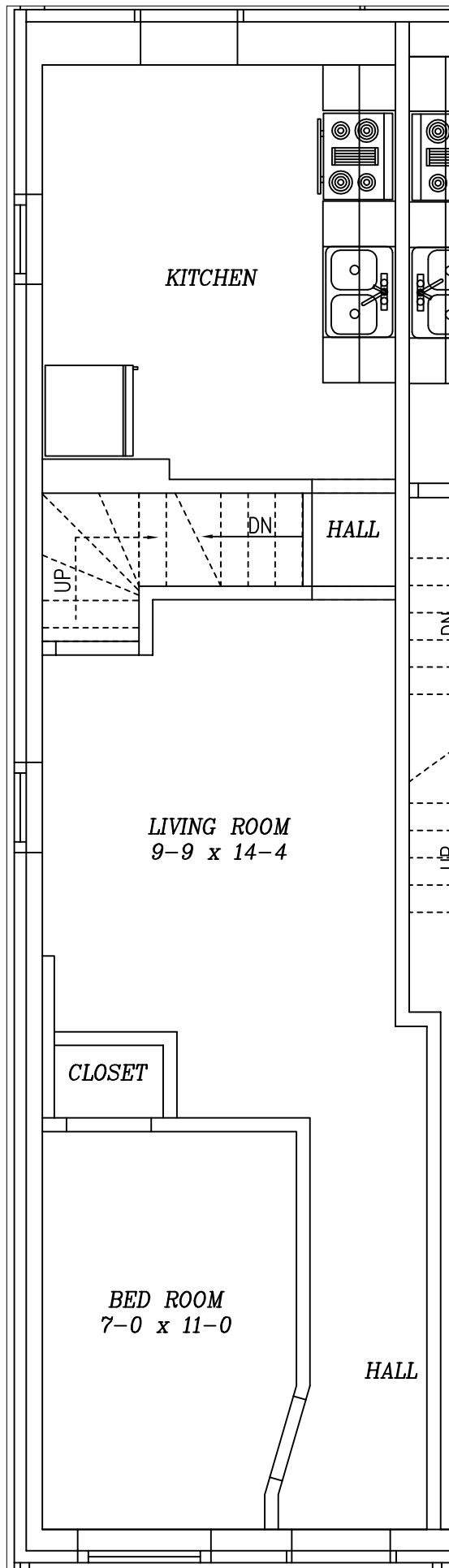
1070 Vine Ave. First Floor Not to Scale
