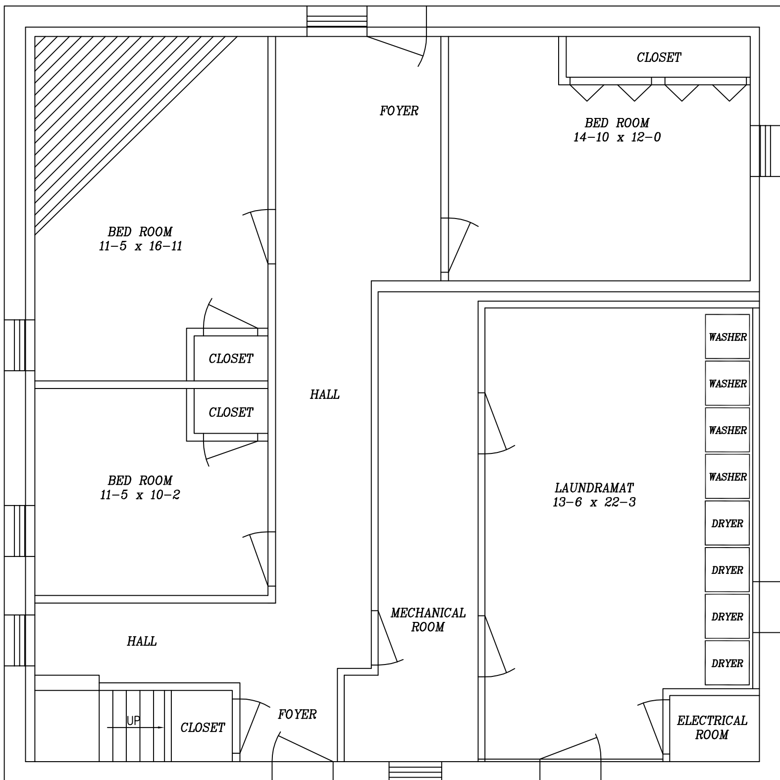
1032 W Fourth St: First Floor Not to Scale (Gross Living Area 815 sq ft)
