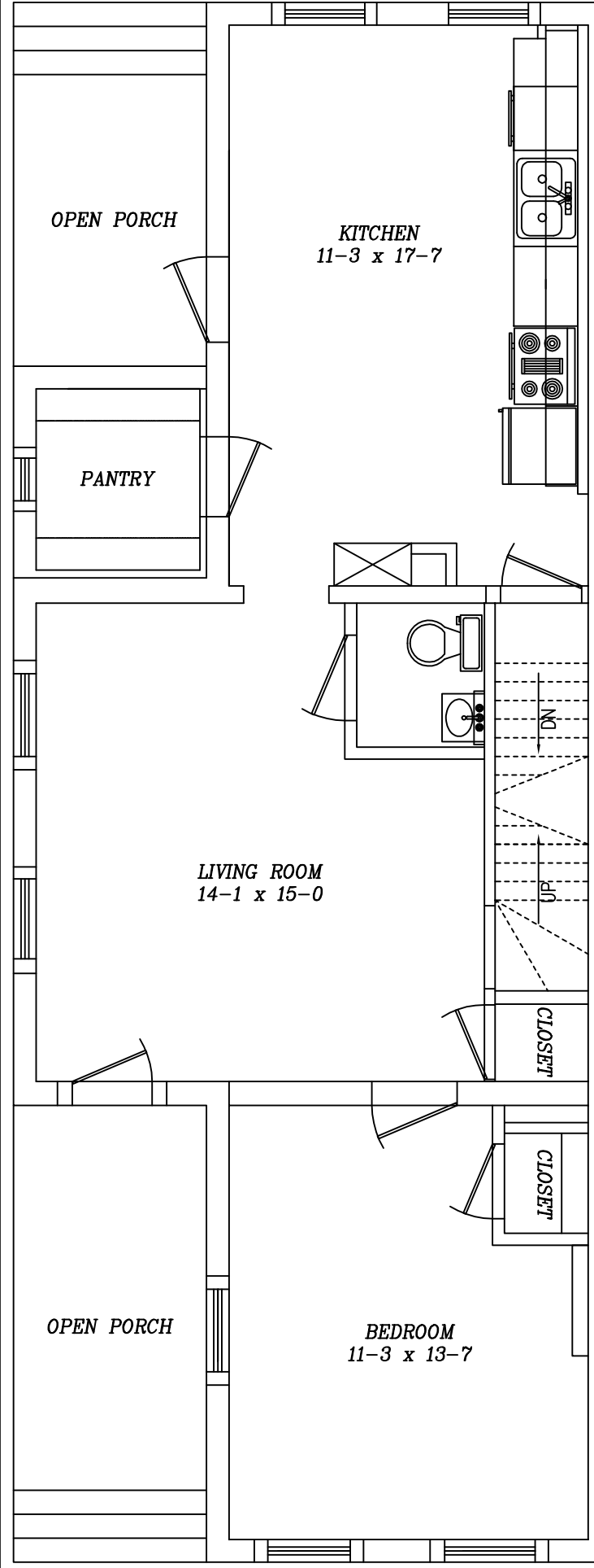
1022 Vine Ave. First Floor Not to Scale
