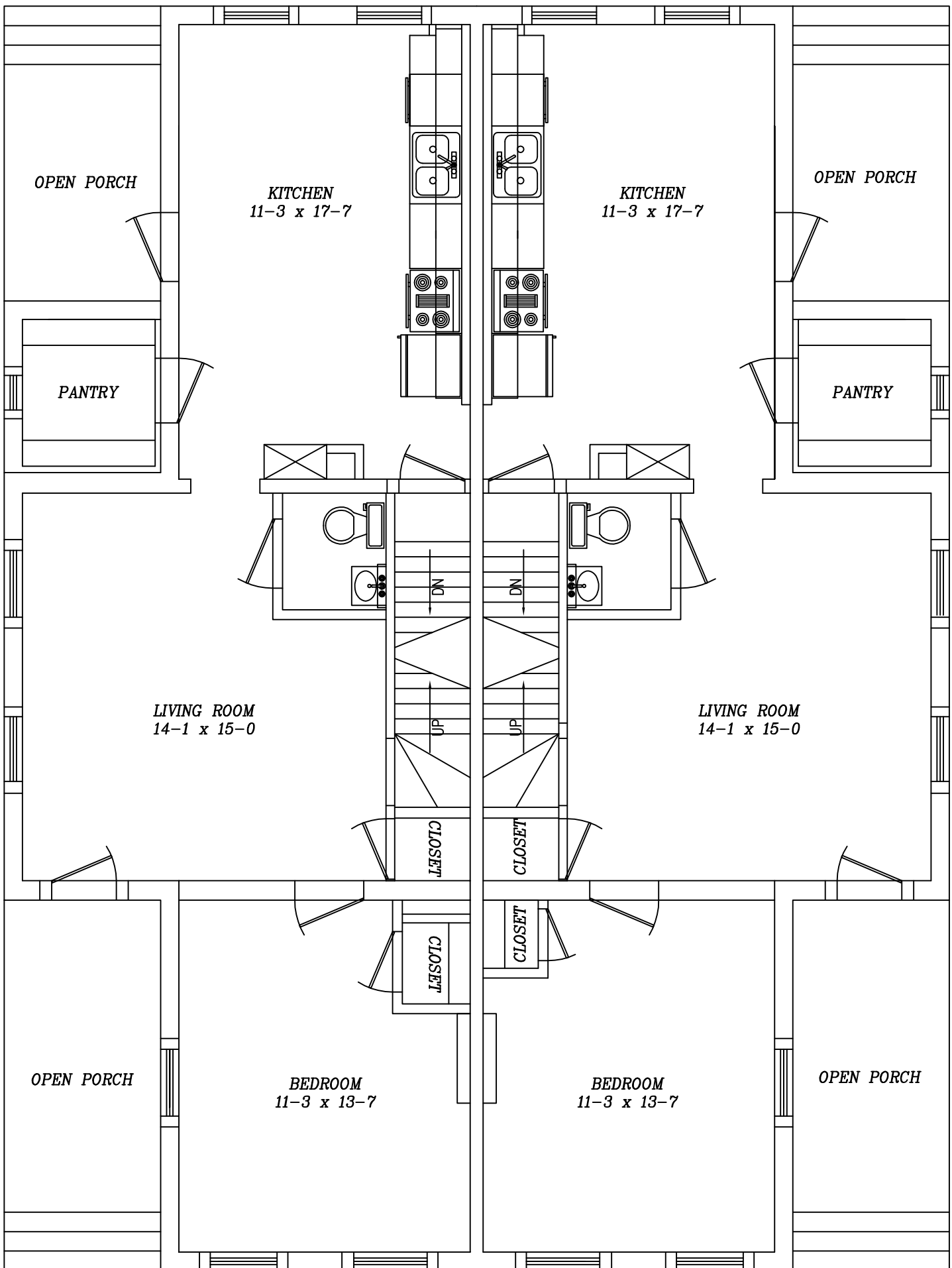
1020-1022 Vine Ave: First Floor Not to Scale (Gross Living Area 1470 sq ft)
