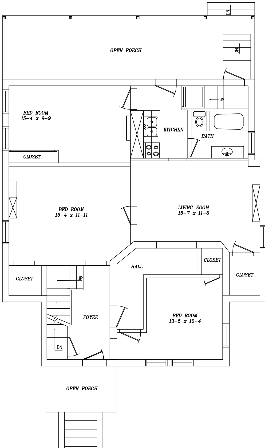
962 Vine Ave: Apt. 1 Not to Scale (Gr Liv Area 1002 sq ft)
